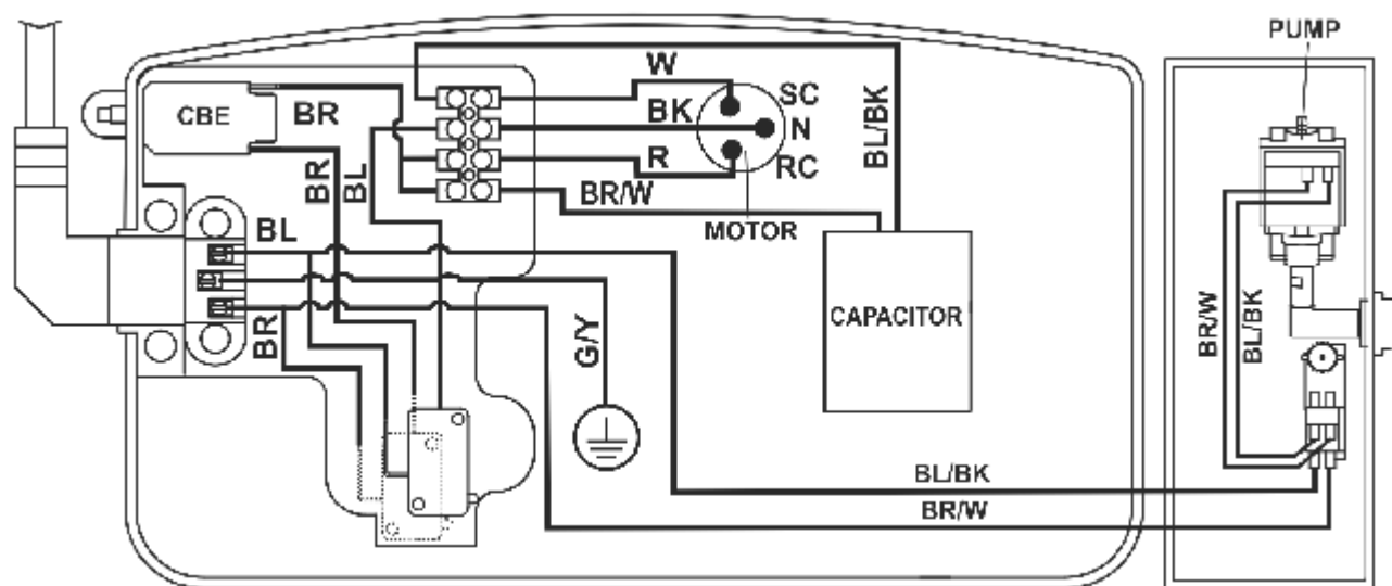
Electrical Layout For P Model
